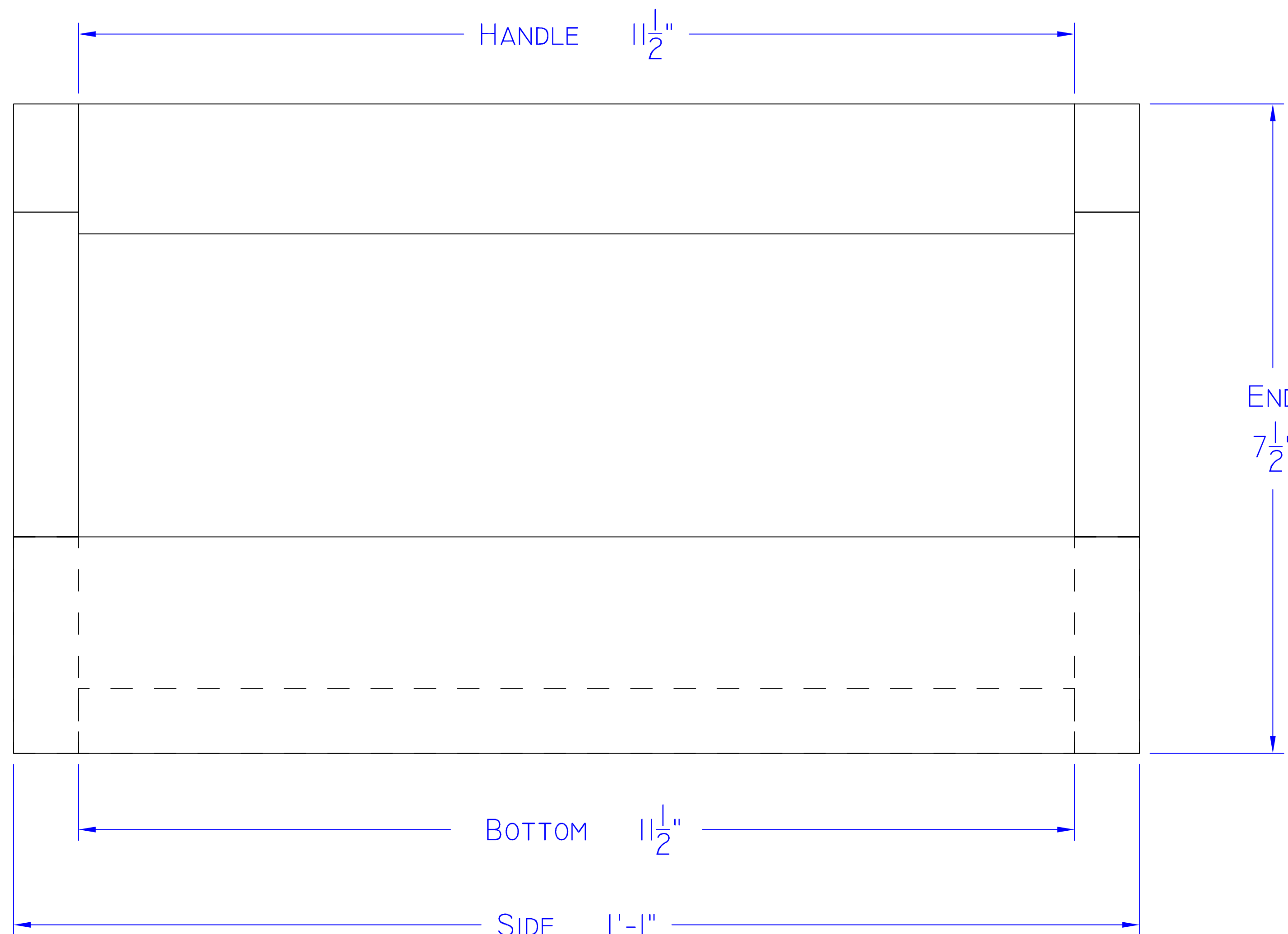
SIDE VIEW
