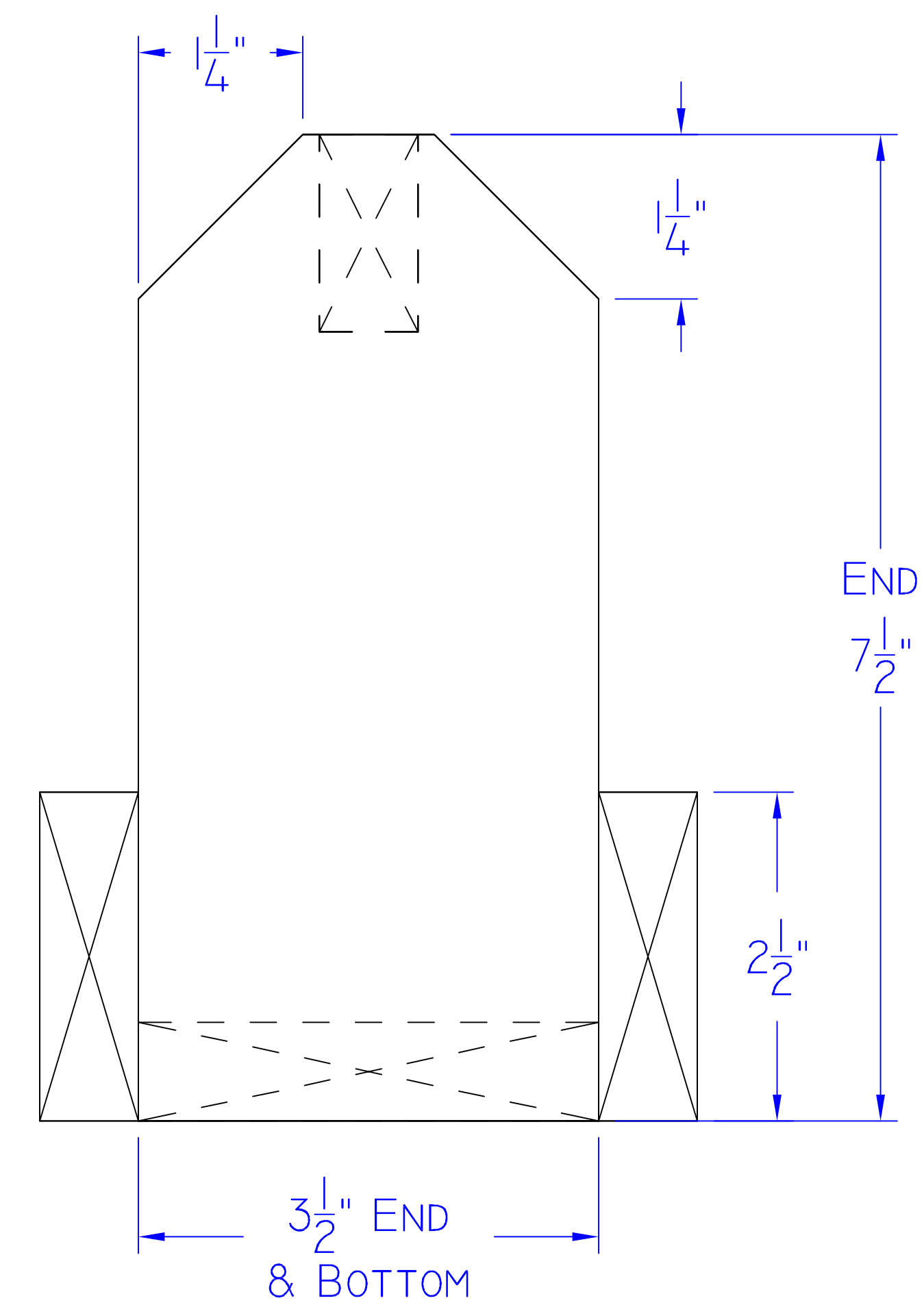
END VIEW
